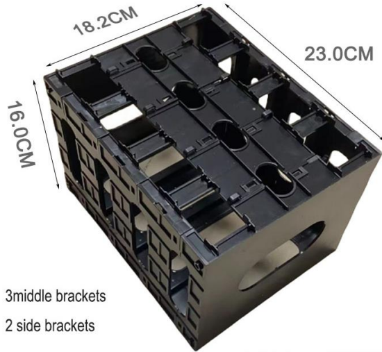
Cell Holder For EVE LF160
